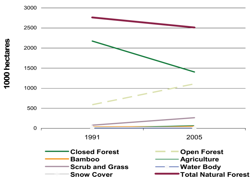
Figure 21: Forest cover changes of China-Kachin border area (1991-2005)
