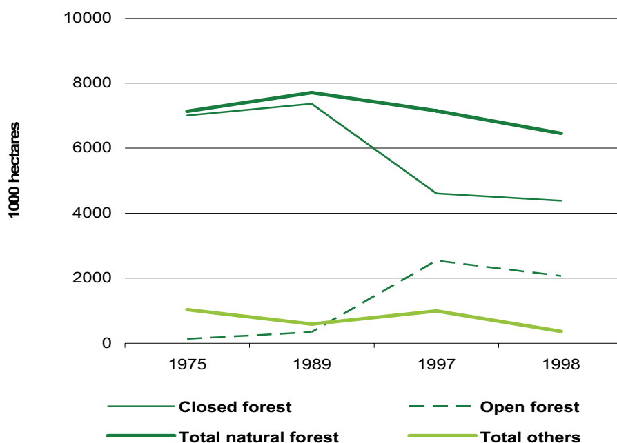
Figure 20: Forest cover assessments of Kachin State (1975-1998)
